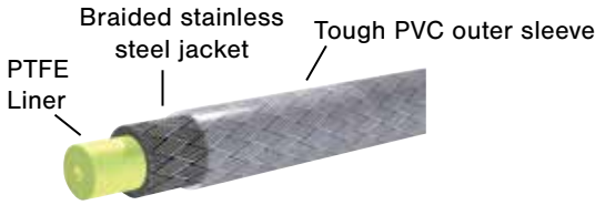
FCB3338 - 15m Reel of Fibrflex®Hose
